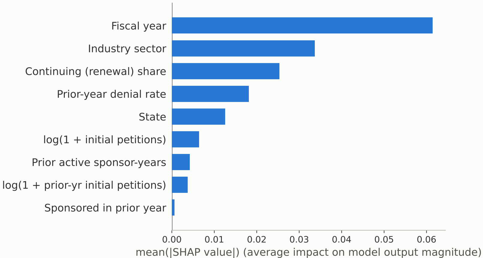
Mean |SHAP| importance on unseen sponsors
