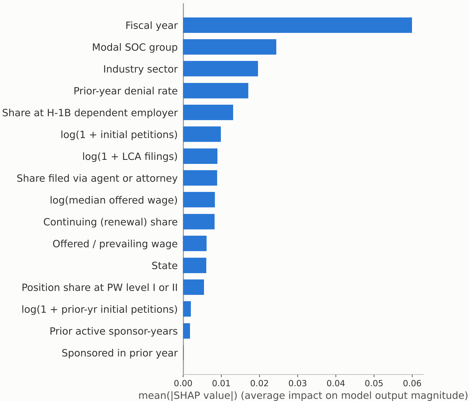
Mean |SHAP| importance with wage data
