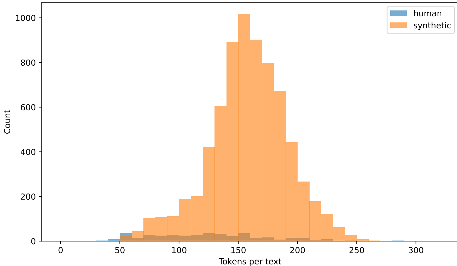
Token length distribution (human vs synthetic)
