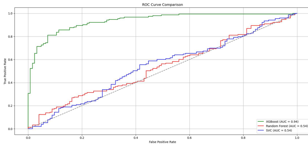
Figure 4.2 1 ROC CURVE
