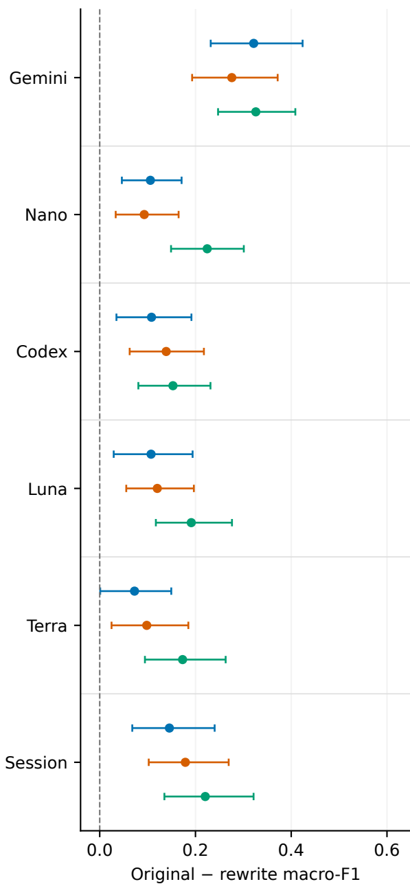
Nearest centroid
