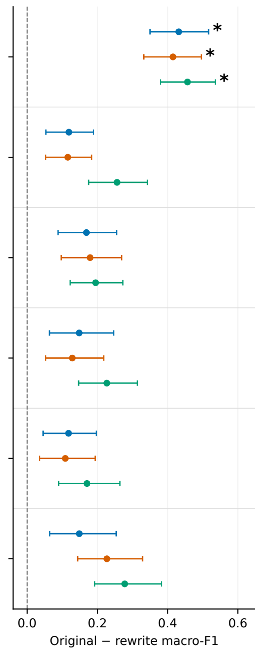
Shrinkage LDA
