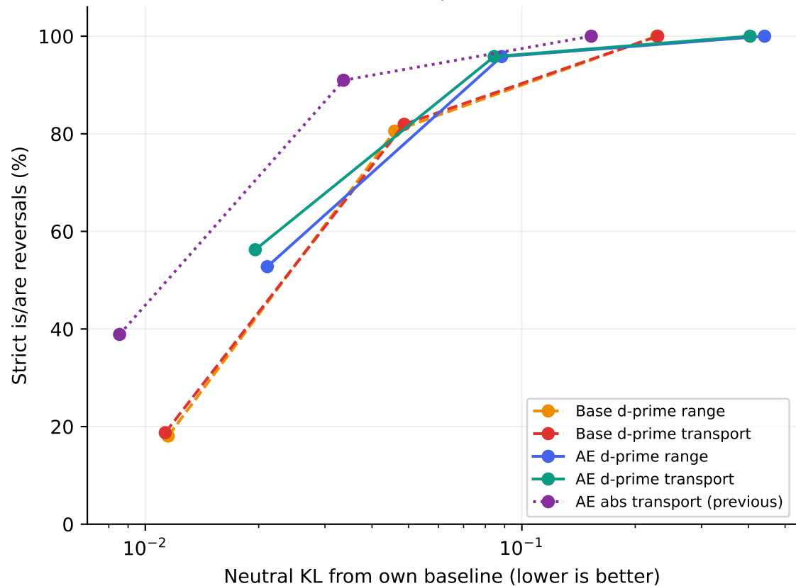
Collateral tradeoff depends on the selector
