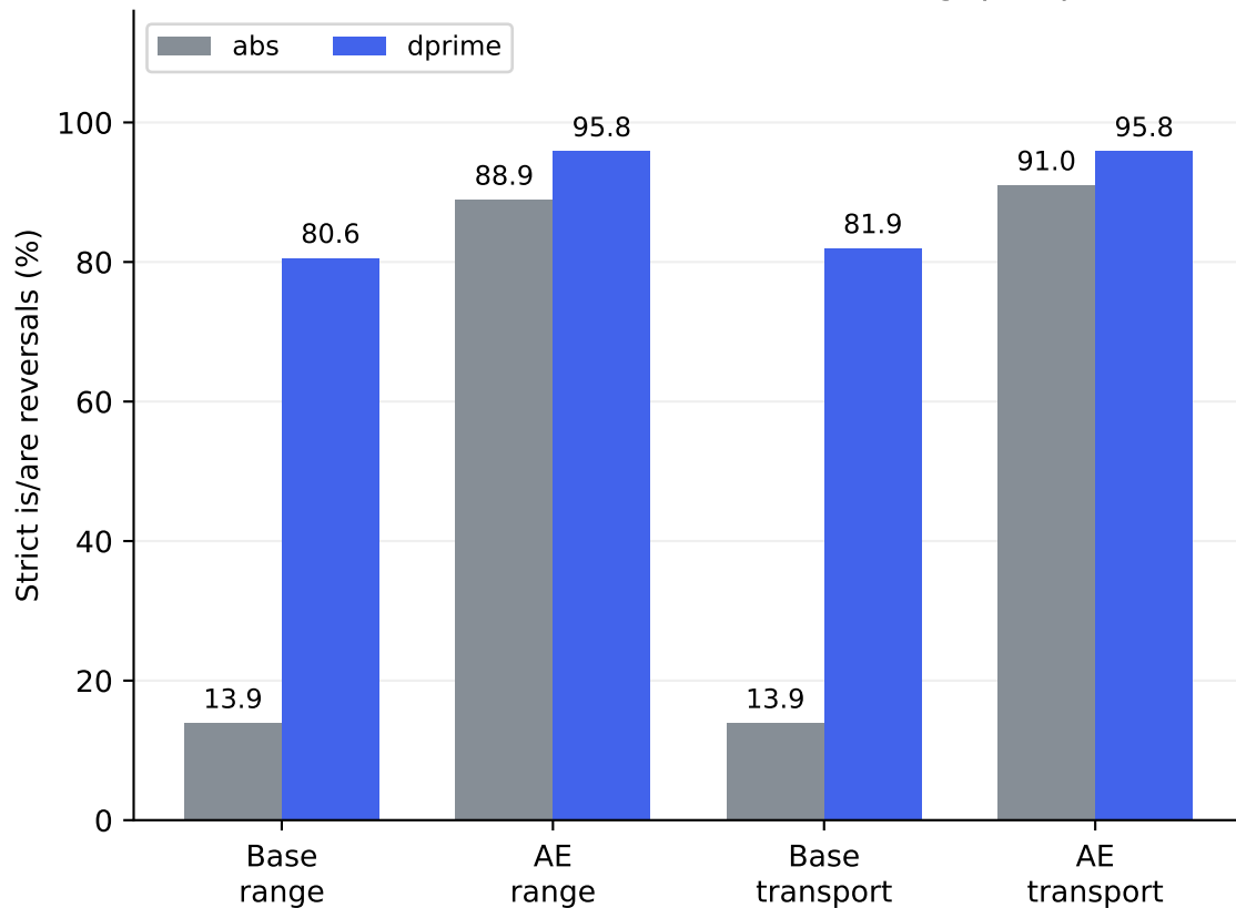
Discriminative selection closes most of the gap ( \alpha = 1 )
