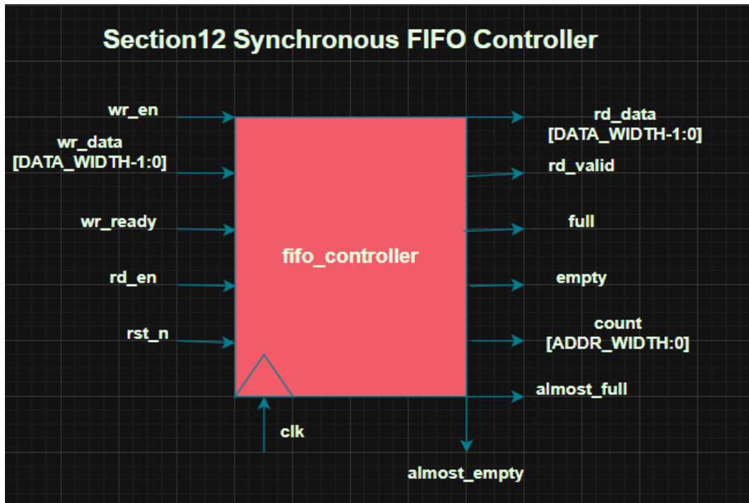
Section12_schematic_diagram
