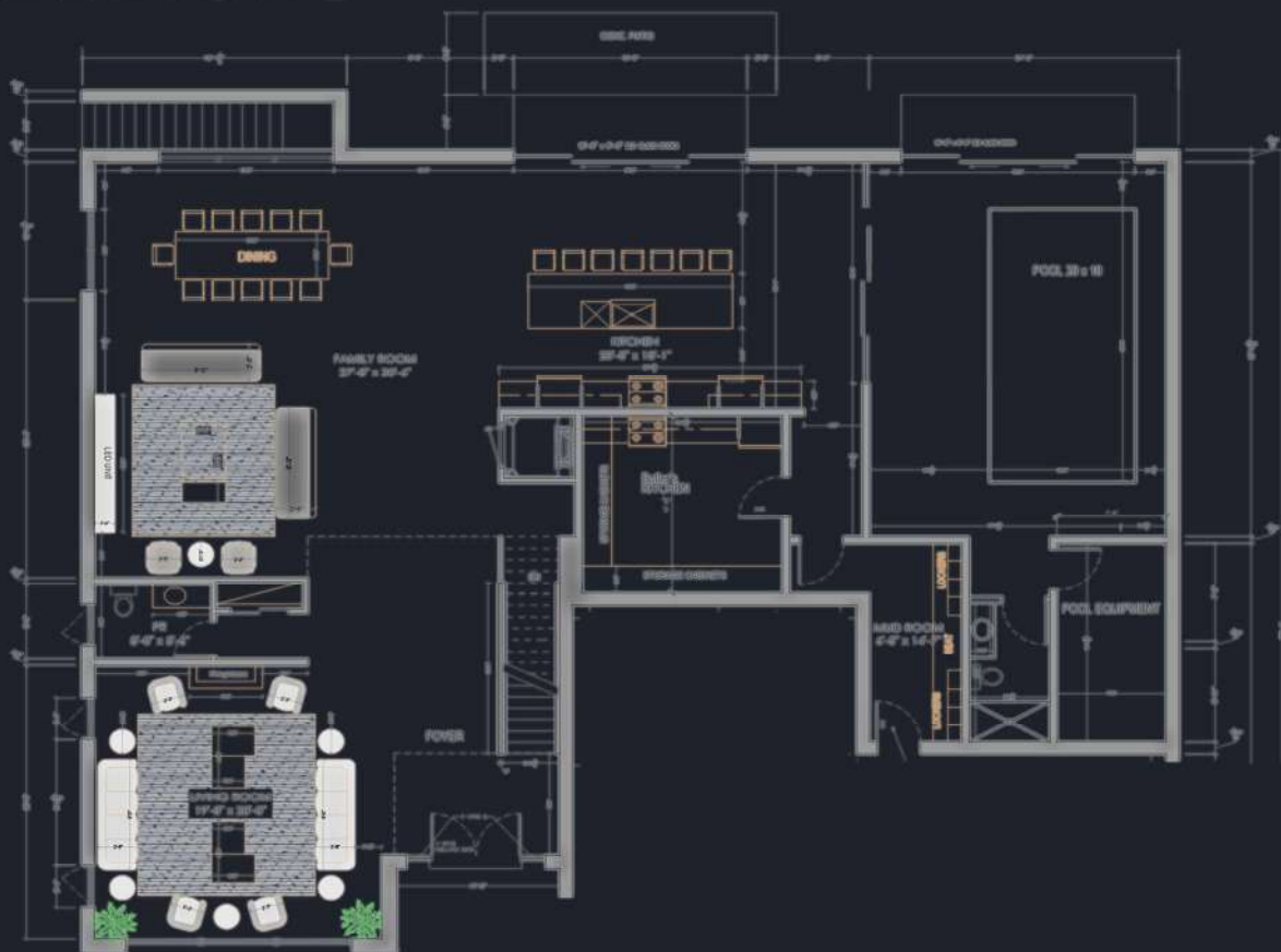
MAIN FLOOR PLAN 3,447 sqft
