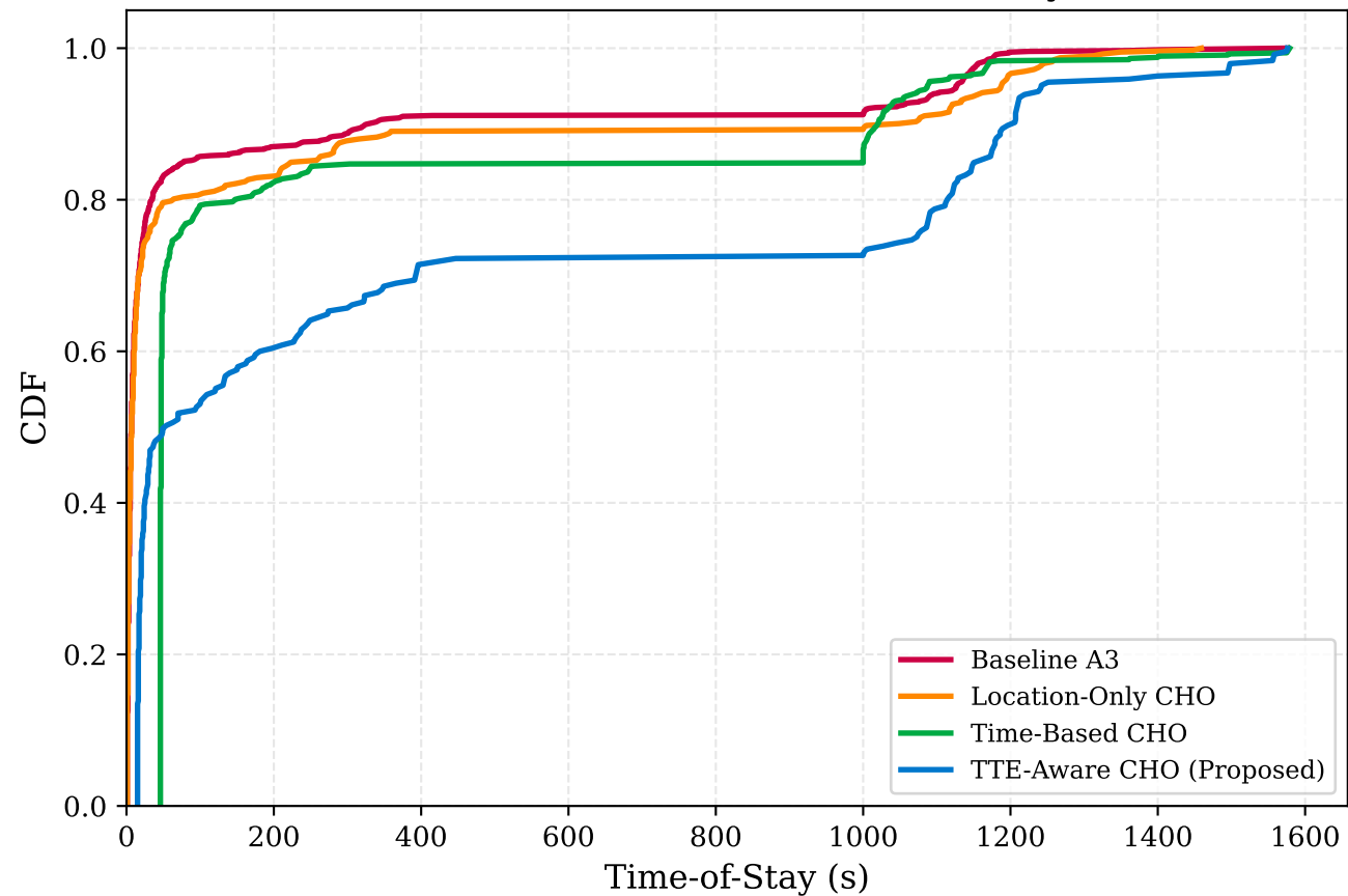
CDF of Post-Handover Time-of-Stay
