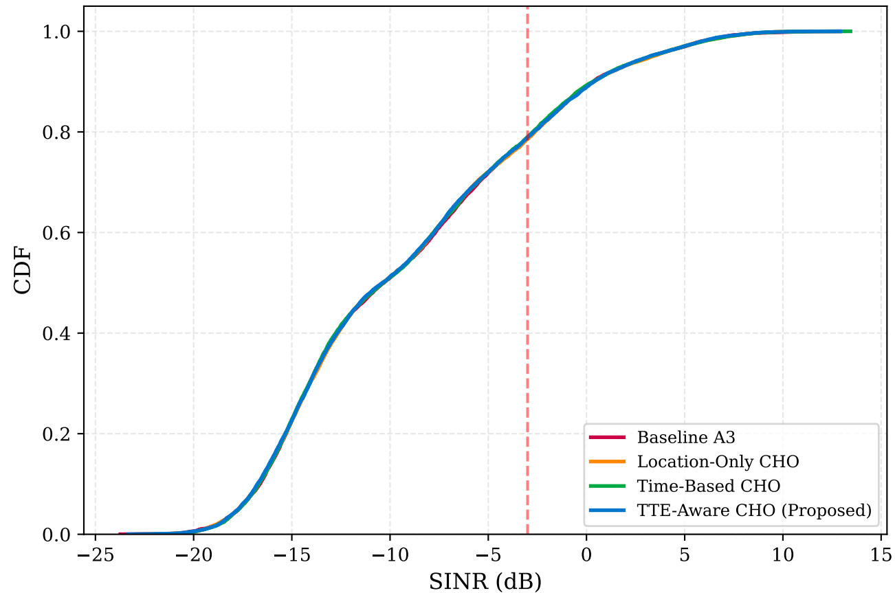
CDF of Measured SINR
