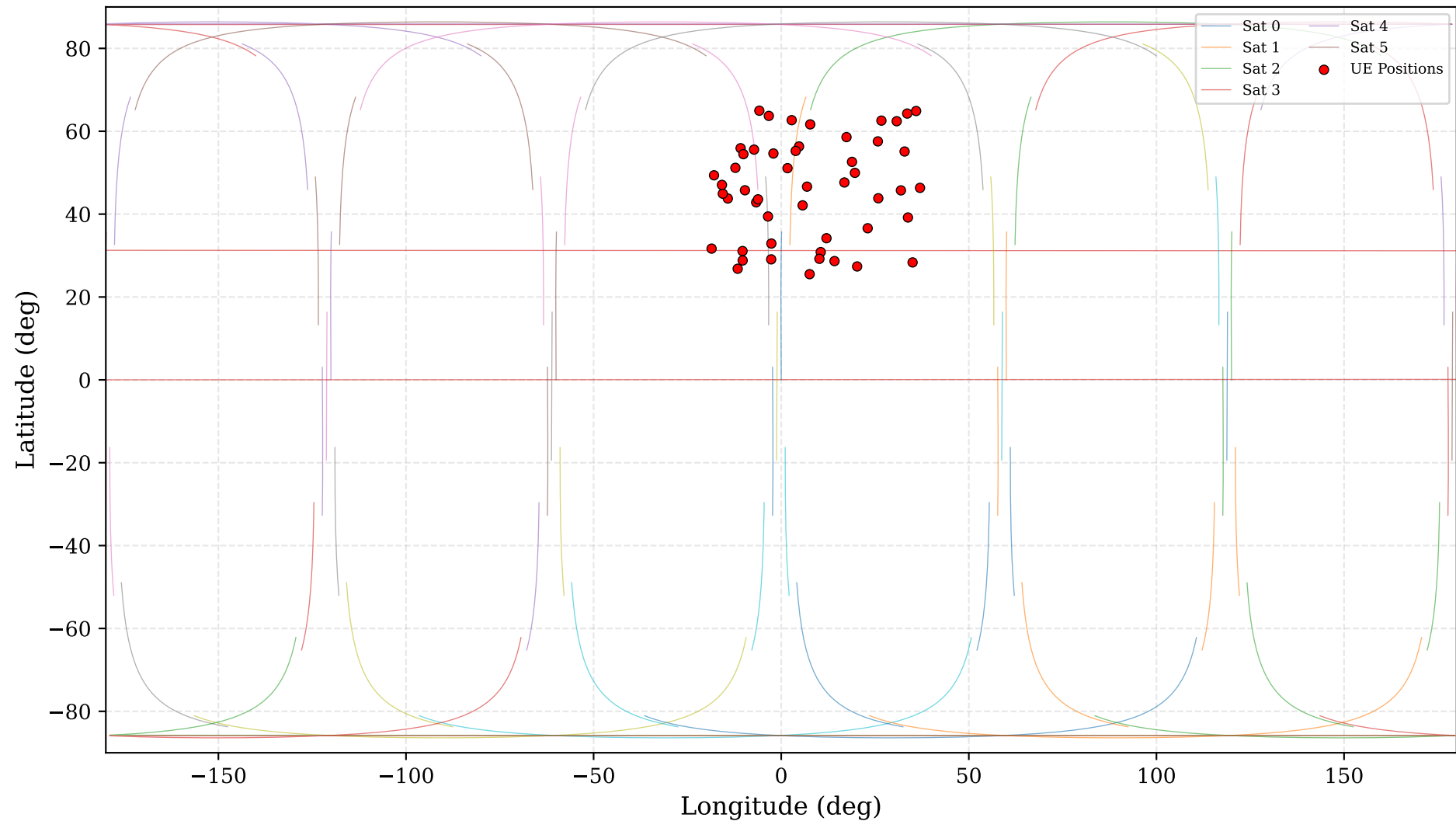
Satellite Ground Tracks & UE Distribution
