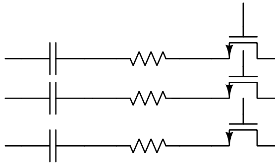
Miller compensation capacitive DAC
