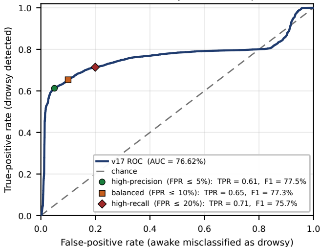
Monitoring-track ROC: lean LDA + causal EMA ( \tau = 600 s) DROZY LOSO, 10 subjects, 14,498 epochs
