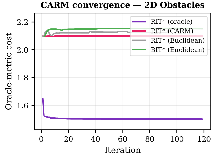
Fig. 10: Convergence comparison under the oracle metric on 2-D Obstacles. RIT* (oracle) converges fastest; CARM achieves lower cost than Euclidean baselines, indicating that the learned metric steers sampling toward better paths.
