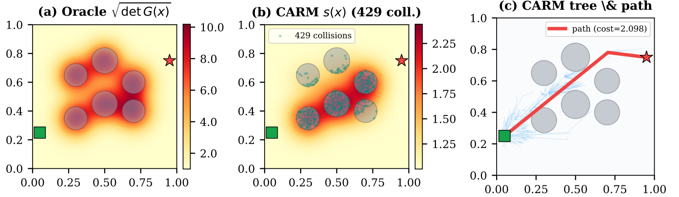
Fig. 11: CARM on 2-D Obstacles. (a) Oracle metric field. (b) CARM-learned scale s(x) after 100 iterations: the field concentrates near obstacle boundaries. (c) Resulting CARM tree and path.
