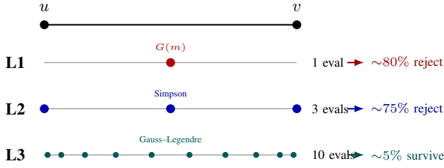
Fig. 5: Cascading edge evaluation. L1 : a single midpoint metric evaluation rejects \sim 80\% of candidate edges. L2 : Simpson’s 3-point rule filters \sim 75\% of survivors. L3 : full 10-point Gauss–Legendre quadrature plus collision checking is applied only to the \sim 5\% of edges that survive both filters.
