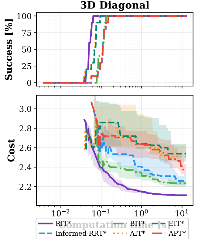
Fig. 9: Anytime performance on the 3-D Diagonal environment with a heavily anisotropic metric ( \kappa \approx 6 ). RIT* finds its first solution almost as fast as AIT*/EIT* (which use cheap Euclidean heuristics) and converges to a strictly lower cost than every baseline; BIT* is second-best but \sim 5\% higher in final cost.
