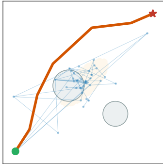
t = 150 : converged
