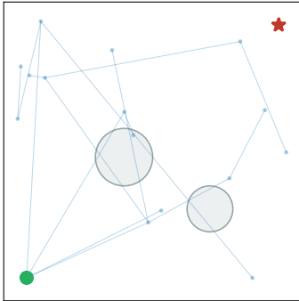
t = 0 : explore
