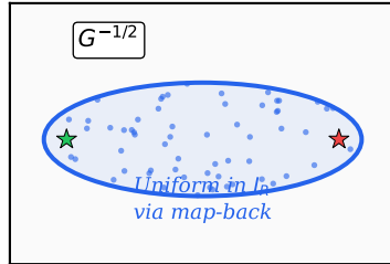
(c) Sample in whitened, map back to original
