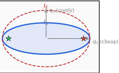
(a) Original space I_R is ellipsoidal
