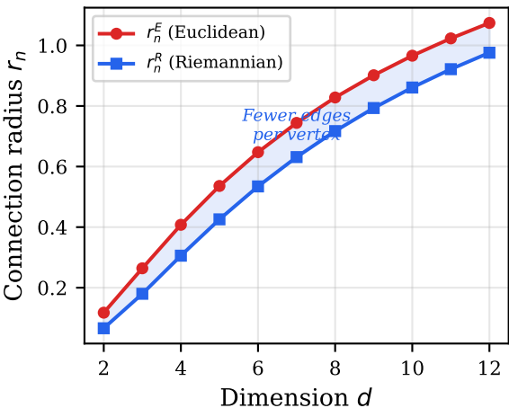
Metric-adapted radius ( \kappa = 10, n = 1000 )
