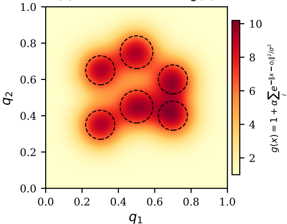
(a) Metric scalar field g(x)
