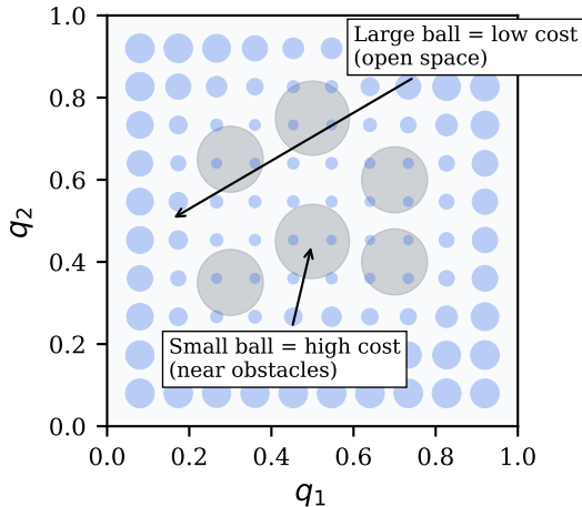
(b) Unit metric balls \{v : v^T G(x) v \leq 1\}
