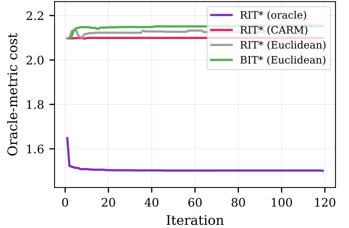
Fig. 8: Convergence comparison under the oracle metric on 2-D Obstacles. RIT* (oracle) converges fastest; CARM achieves lower cost than Euclidean baselines, indicating that the learned metric steers sampling toward better paths.
