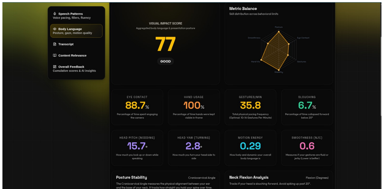
Figure 4.6: TC05-CV Analysis Dashboard
