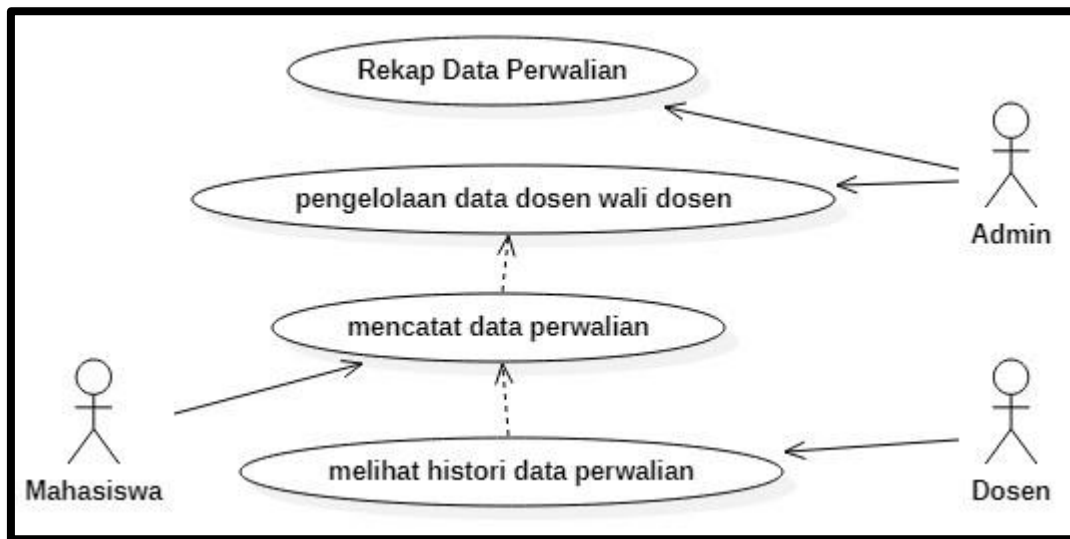
Gambar 1. Usecase sistem perwalian
