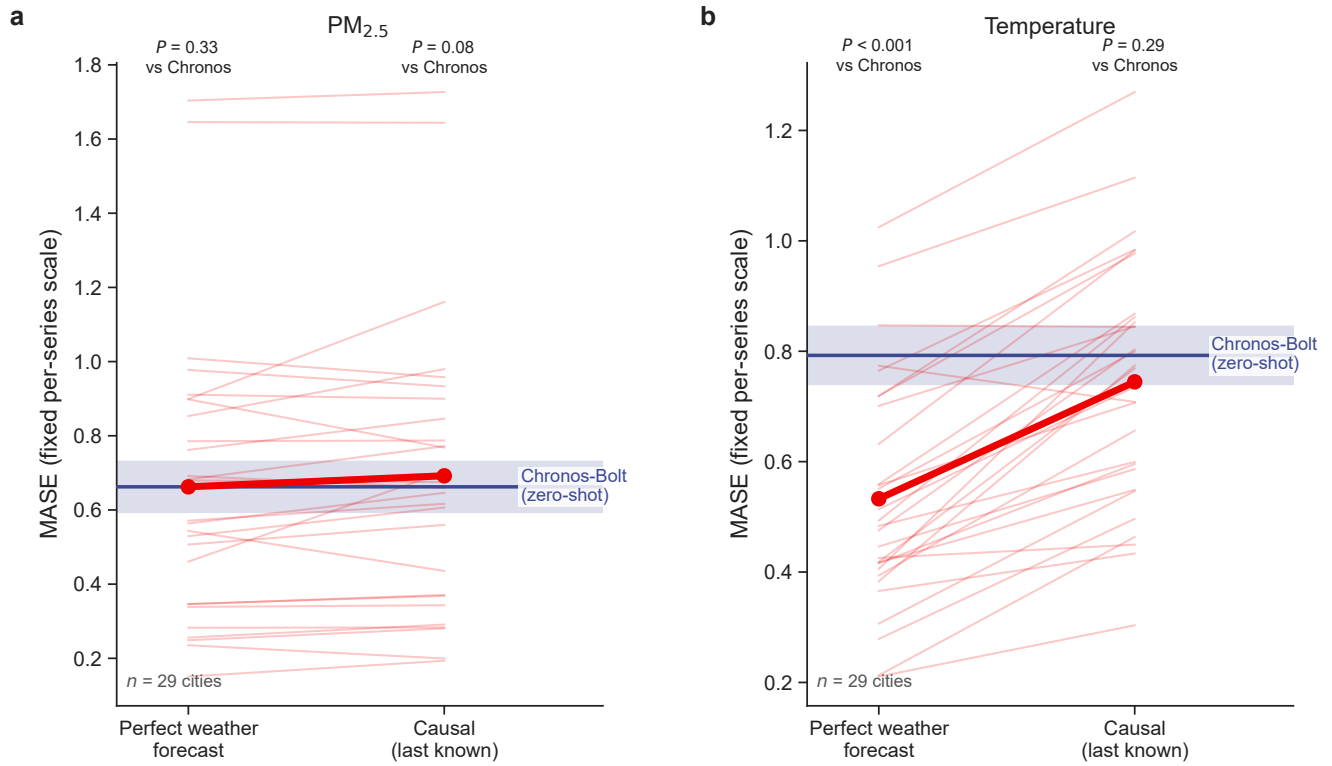
Figure 3. The specialist’s temperature edge requires a perfect weather forecast. Per-city LightGBM MASE with perfect-foresight covariates (left ticks) versus causal, last-known covariates (right ticks), n = 29 cities per panel; bold line = panel mean; horizontal band = zero-shot Chronos-Bolt panel mean \pm s.e.m. across cities. On-panel P -values are paired Wilcoxon signed-rank tests of LightGBM against Chronos-Bolt. (a) \text{PM}_{2.5} : foresight is worth \sim 0 (0.662 vs 0.692; both statistically indistinguishable from the foundation model). (b) Temperature: removing foresight moves the specialist from 0.533 (26/29 city wins, P = 1.4 \times 10^{-6} ) to 0.745 (16/29, P = 0.29 , not significant) against the foundation model at 0.792.
