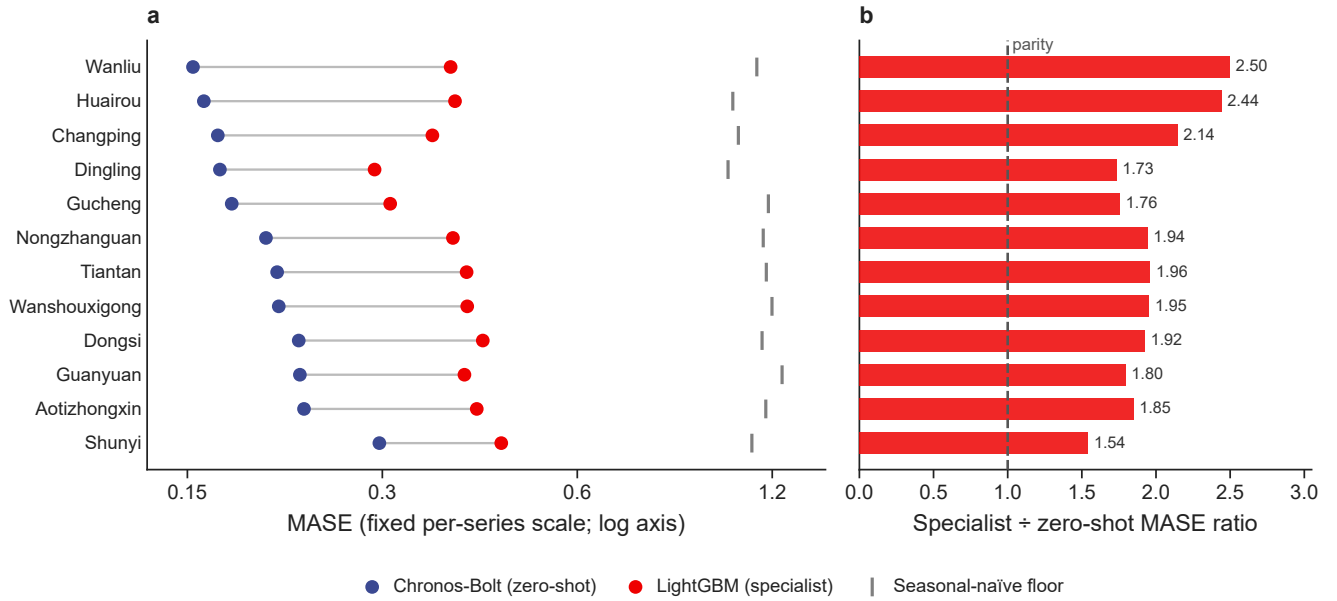
Figure 4. Beijing multi-station depth check. (a) Per-station MASE at the 12 UCI Beijing multi-site stations (six-fold backtest, after the pre-specified value-sanitization step; Methods). Zero-shot Chronos-Bolt (0.153–0.297) beats the LightGBM specialist (0.292–0.458) at 12/12 stations; the seasonal-naïve floor spans 1.03–1.24. (b) Specialist-to-foundation-model MASE ratio per station (same station order); the dashed line marks parity. The advantage is uniform across the metropolitan network rather than driven by a subset of stations, so the panel-level tie is not an averaging artifact.
