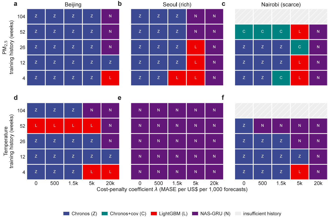
Figure 5. Cost-adjusted deployment winner maps (causal covariates). Winning tier under the objective MASE + \lambda \cdot \text{USD}/1,000 \text{ forecasts} , per training-history regime (rows: weeks of history) and cost-penalty coefficient \lambda (columns), for Beijing, Seoul, and Nairobi in both domains (a-f), using the deployable causal (last-known) covariates. PM2.5 maps are dominated by the Chronos family (21/25, 14/25, and 13/20 cells). Under causal covariates the temperature maps no longer favour the specialist: the Chronos family and NAS-GRU take most cells (e.g. Beijing 15/25 Chronos vs 6/25 specialist; Seoul 25/25 NAS-GRU), a marked shift from the perfect-foresight version (Supplementary Fig. S1), consistent with the ablation (Fig. 3). Sweeping electricity price over 0.05–0.30 USD/kWh and PUE over 1.0–2.0 flips no cells at the central assumption and at most 40% at the most extreme corners (Supplementary Table S12). Cell letters duplicate the colour coding for grayscale readers.
