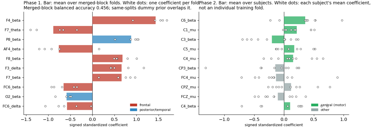
Figure 3: Signed standardized logistic-regression coefficients from the saved JSON. Bars are means. Left, Phase 1: white dots are the coefficient from each merged-block training fold. Right, Phase 2: white dots are subject-mean coefficients, one per subject, not individual training-fold coefficients. The largest Phase 2 mean absolute weights are C6_beta, C1_mu, C3_beta, C5_mu, and C4_mu. The Phase 1 model’s balanced accuracy is 0.456 and the same-splits dummy prior is 0.400.
