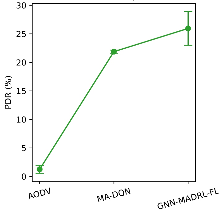
Packet Delivery Ratio
