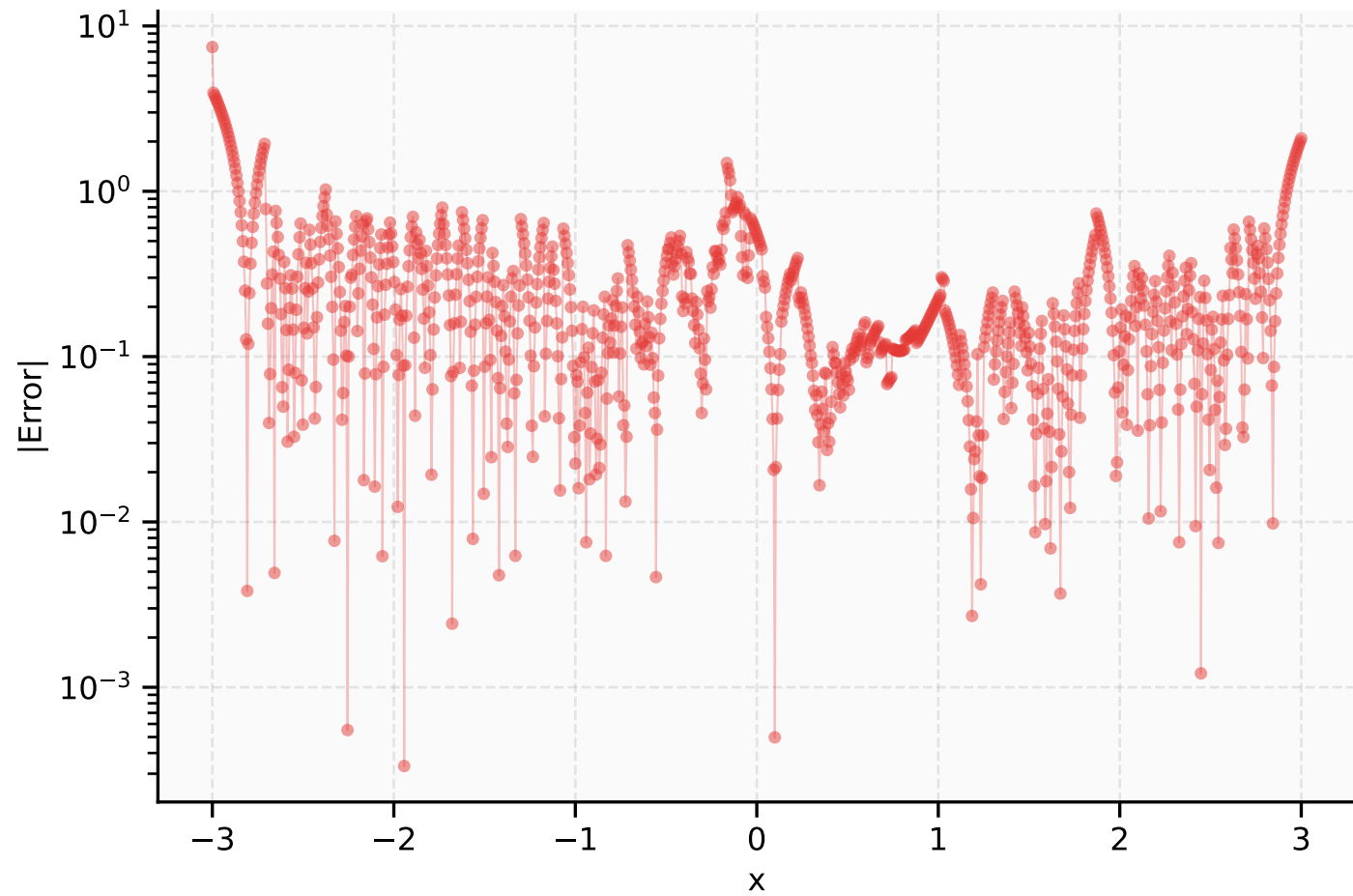
Derivative Error vs Position
