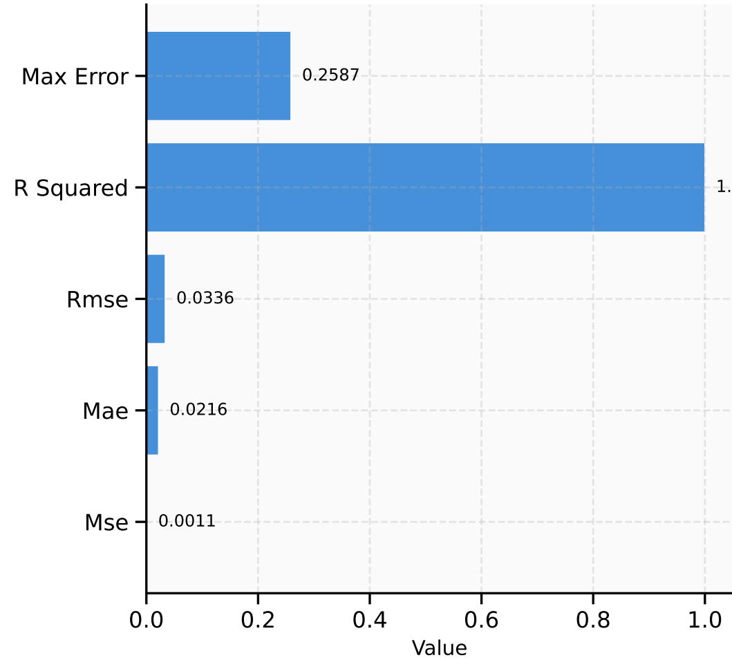
Function Approximation
