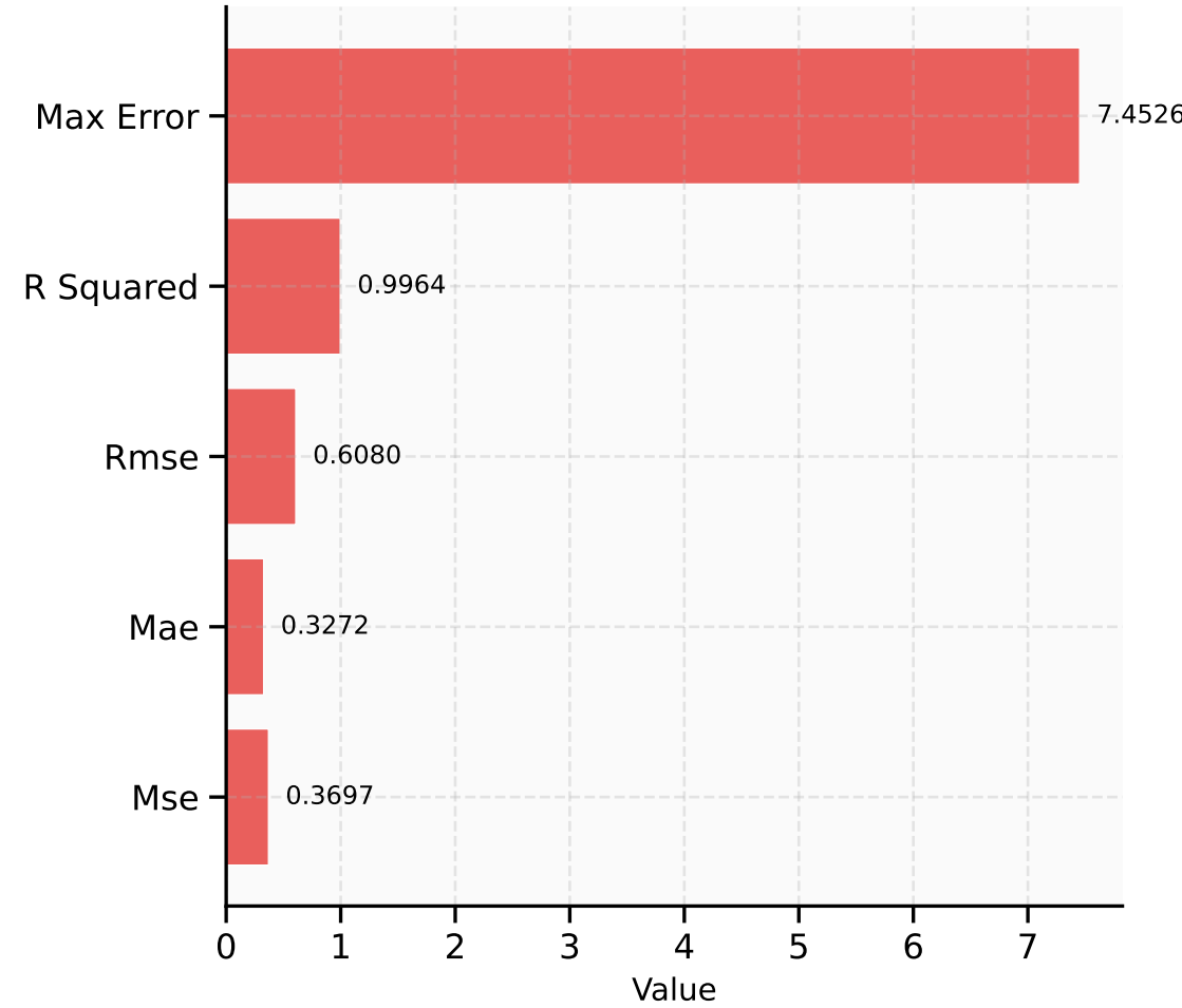
Derivative Estimation
