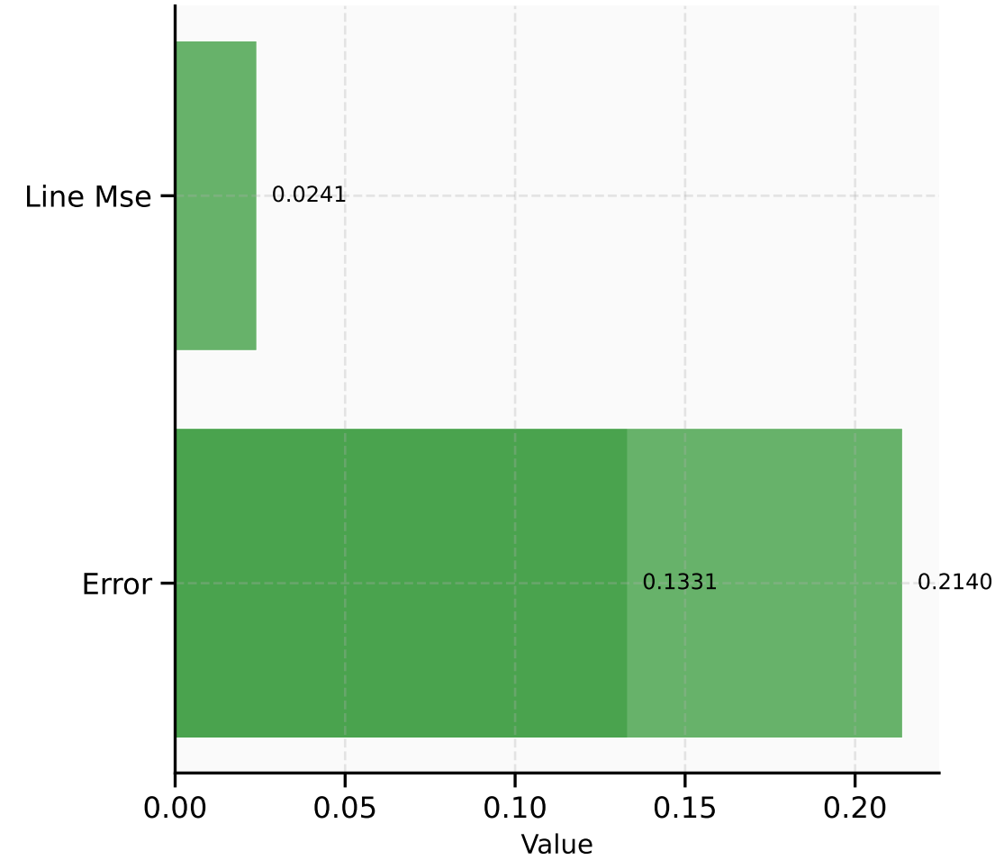
Tangent Line
