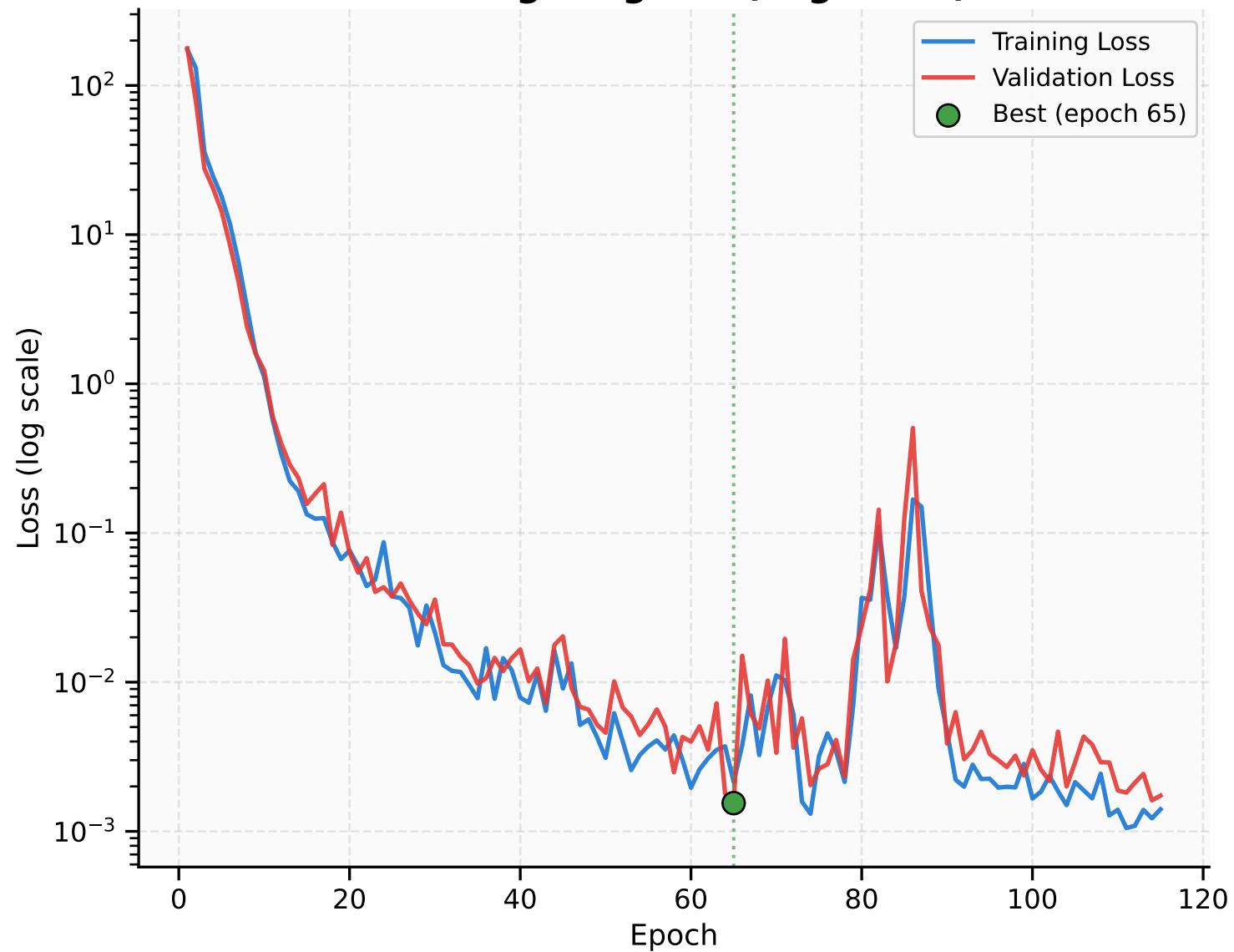
Training Progress (Log Scale)
