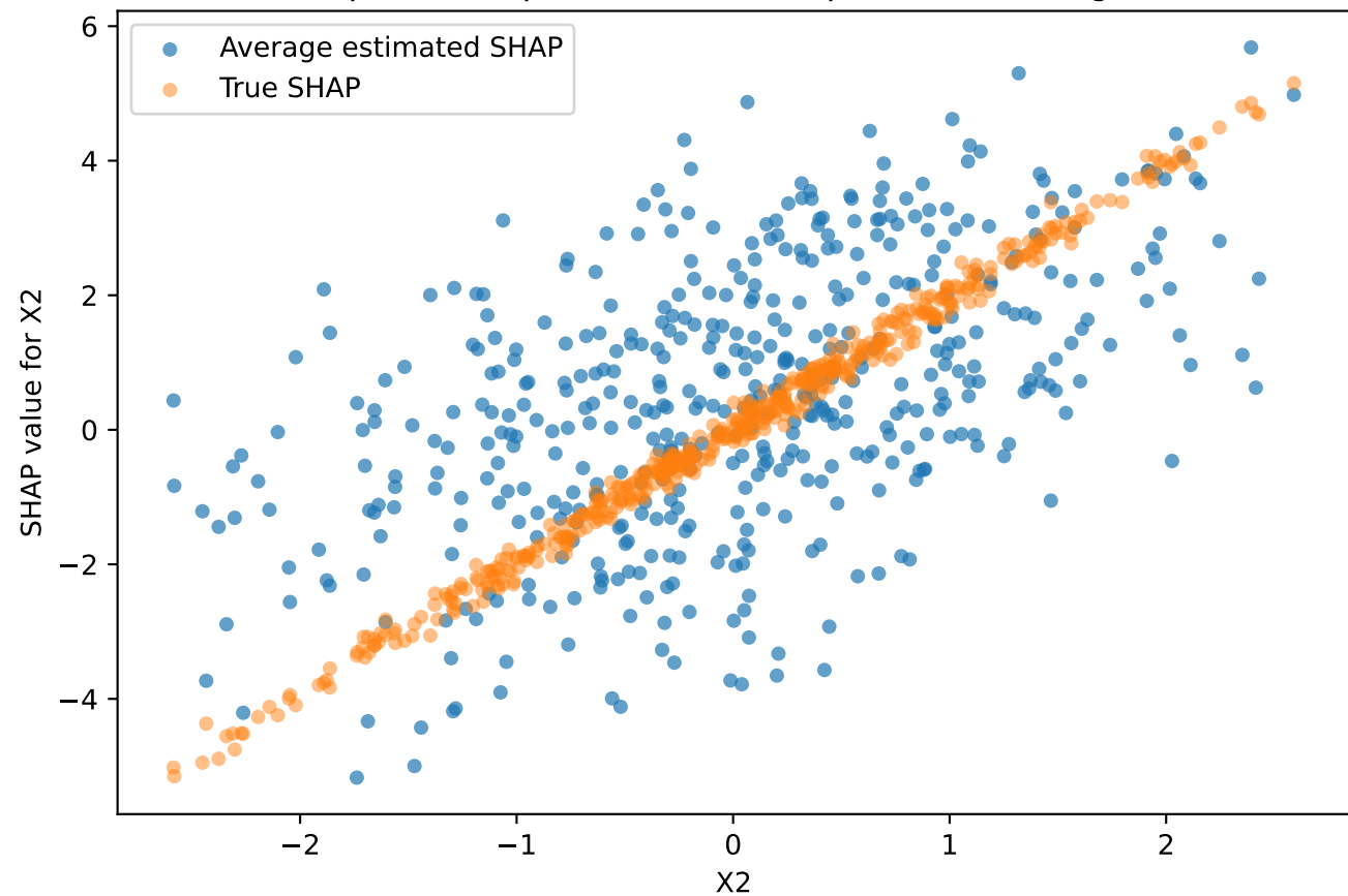
Dependence plot for X2 (100 replications averaged)
