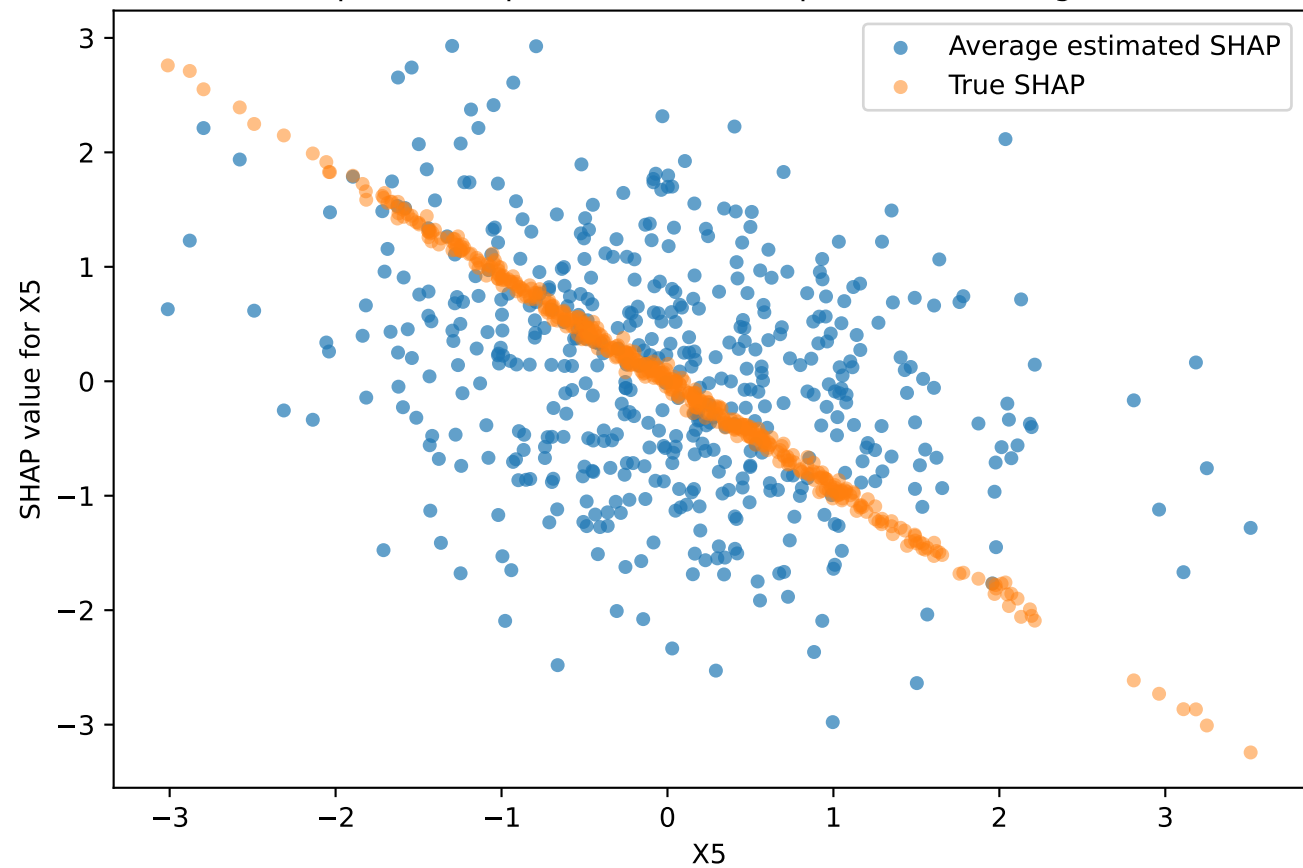
Dependence plot for X5 (100 replications averaged)
