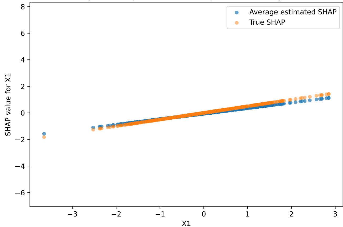
Dependence plot for X1 (100 replications averaged)
