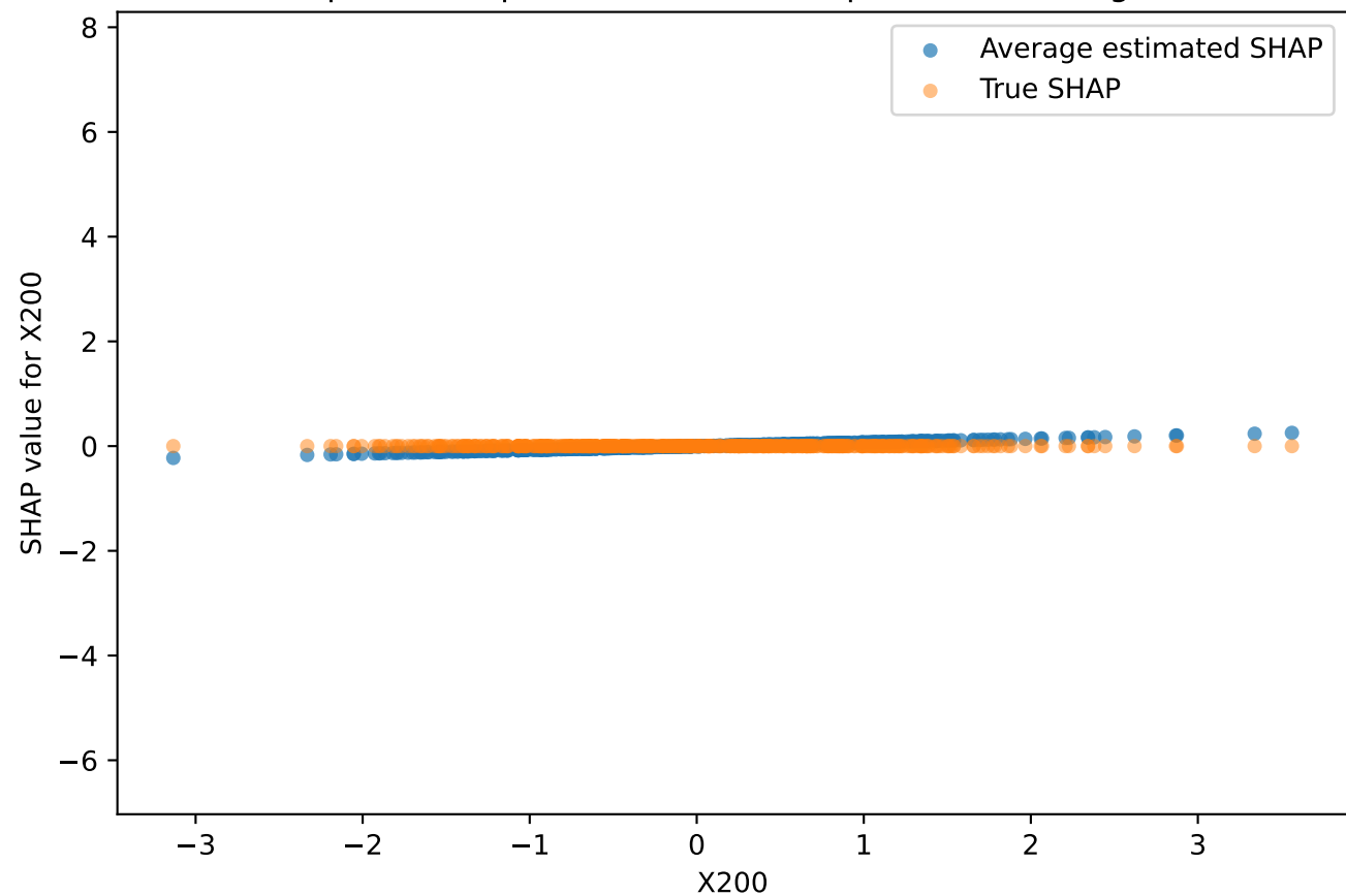
Dependence plot for X200 (100 replications averaged)
