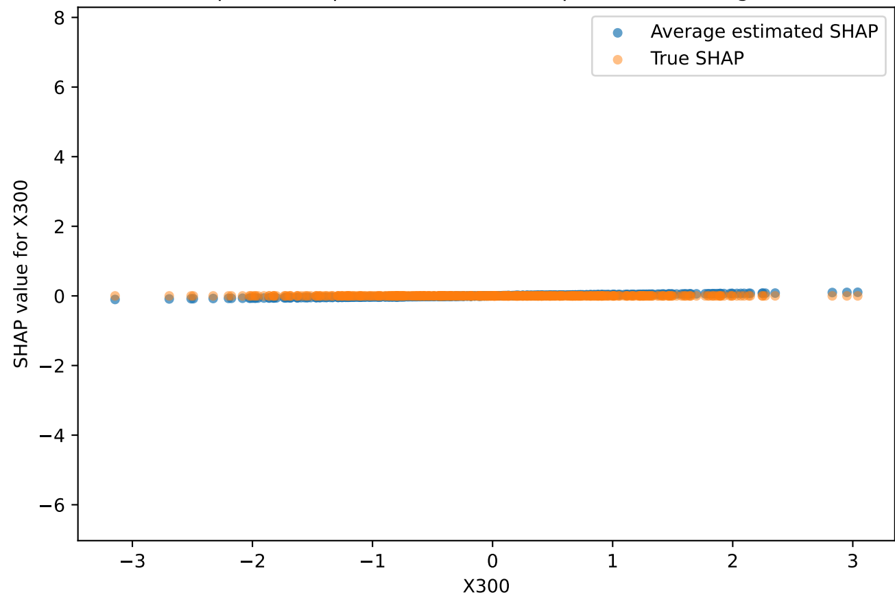
Dependence plot for X300 (100 replications averaged)
