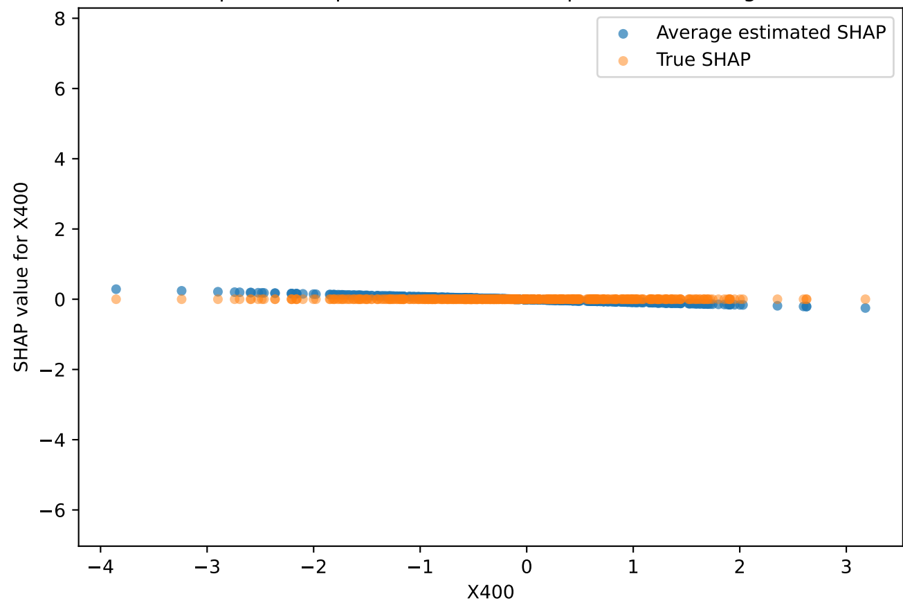
Dependence plot for X400 (100 replications averaged)
