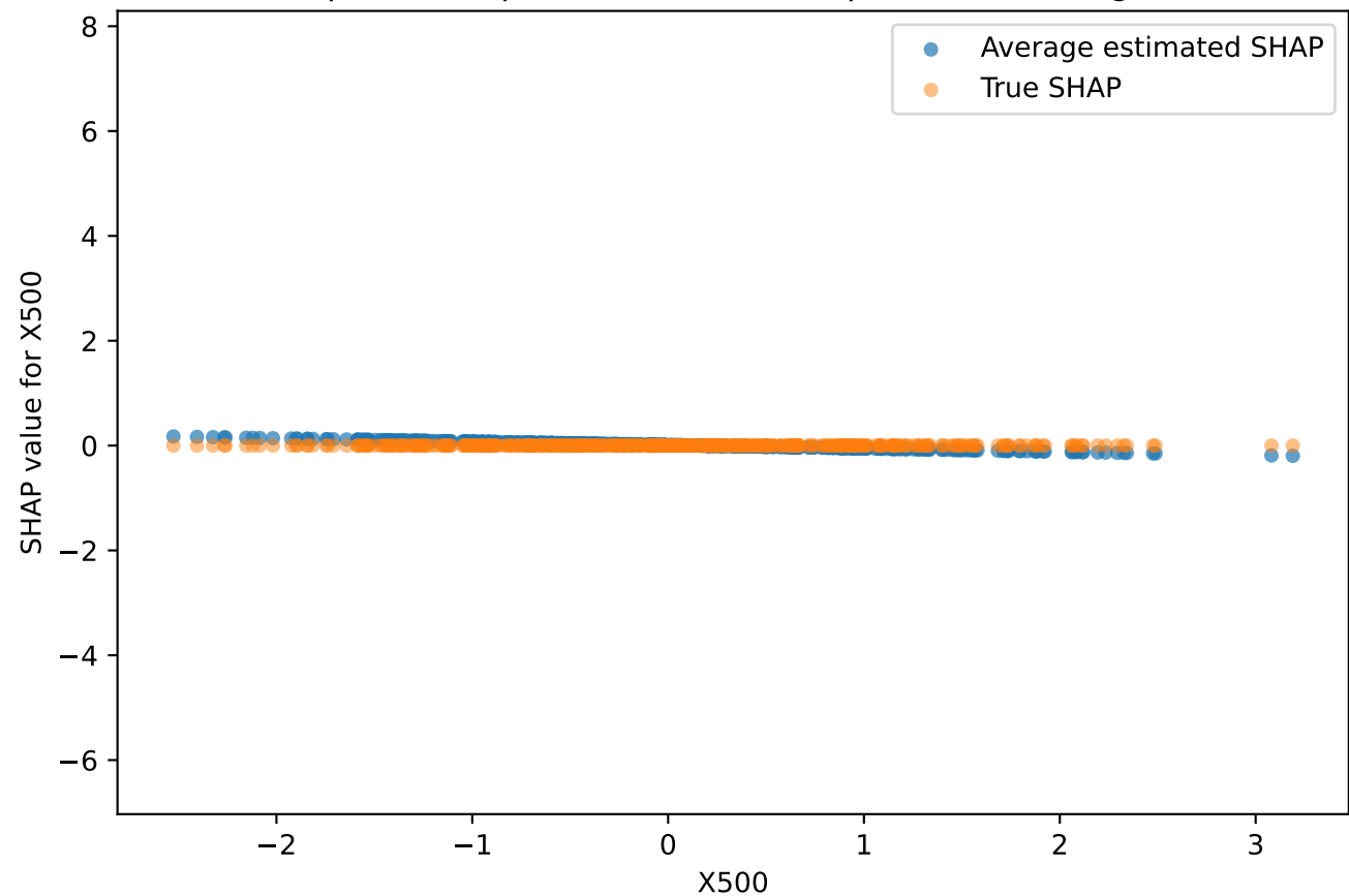
Dependence plot for X500 (100 replications averaged)
