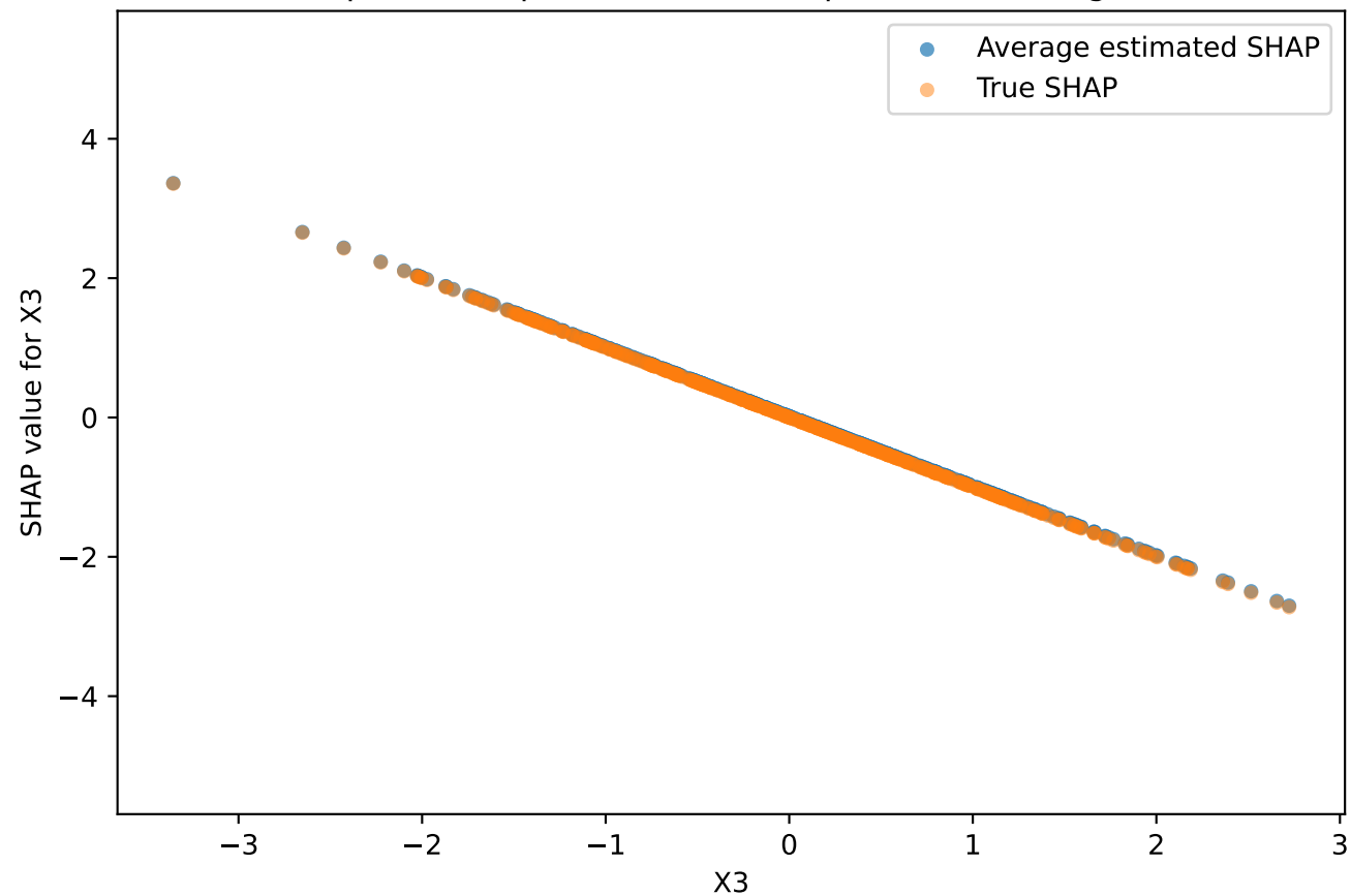
Dependence plot for X3 (100 replications averaged)
