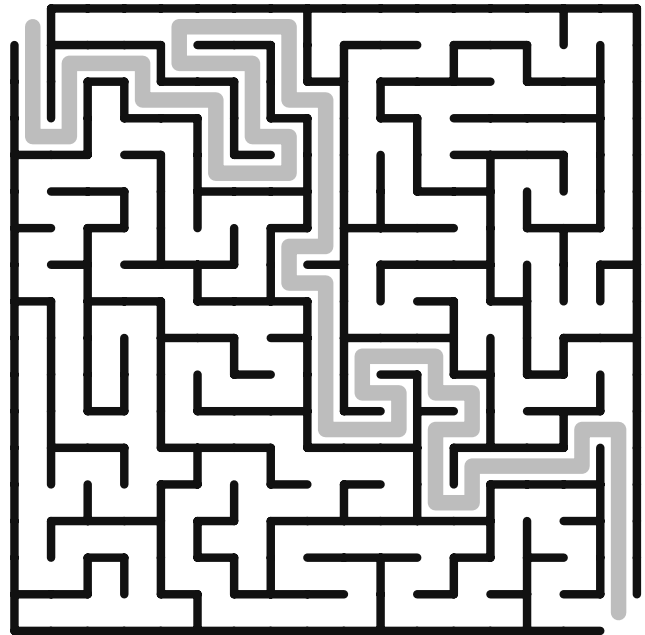
Maze 4
