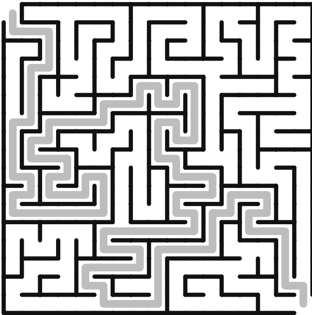
Maze 3
