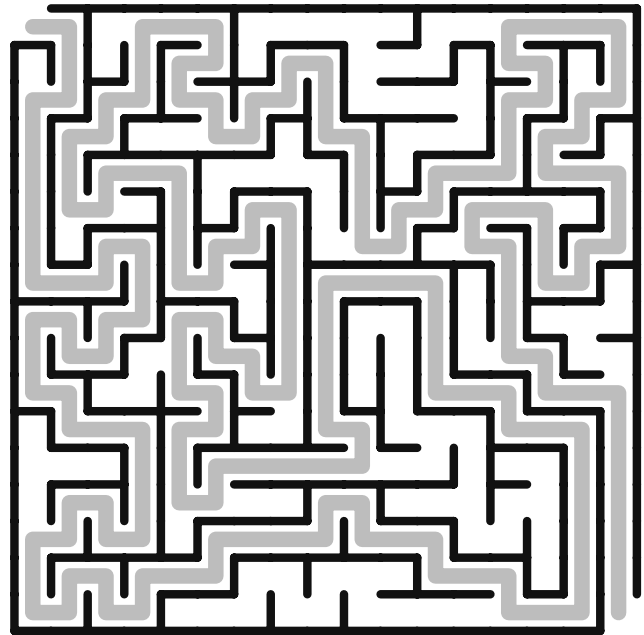
Maze 6
