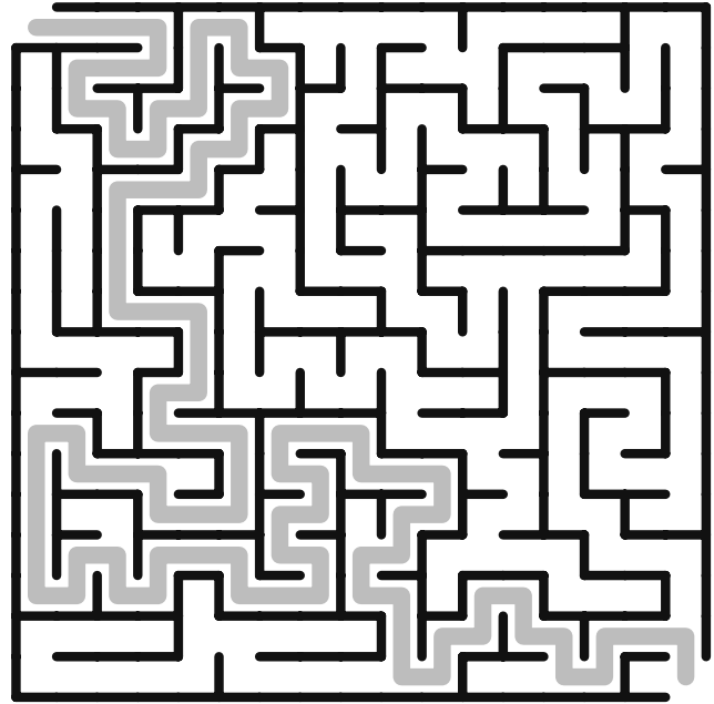
Maze 10
