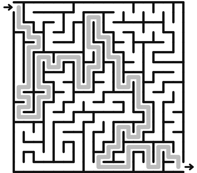
Maze 6
