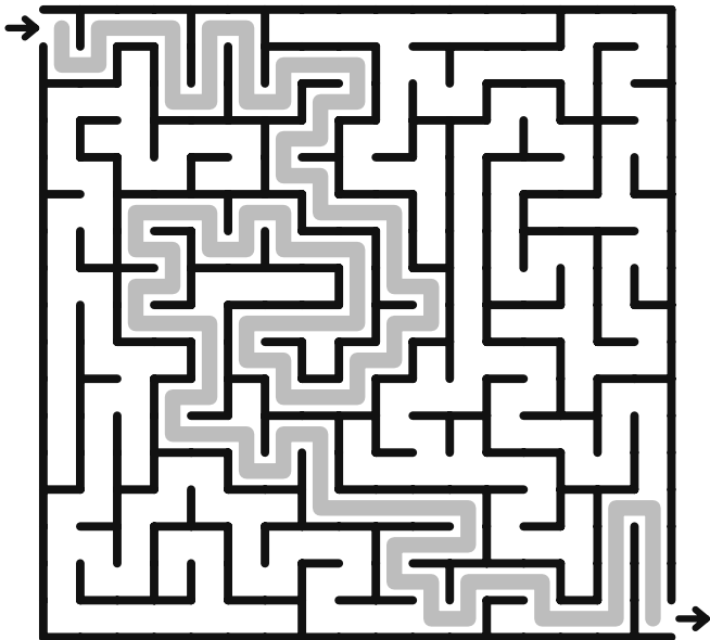
Maze 7
