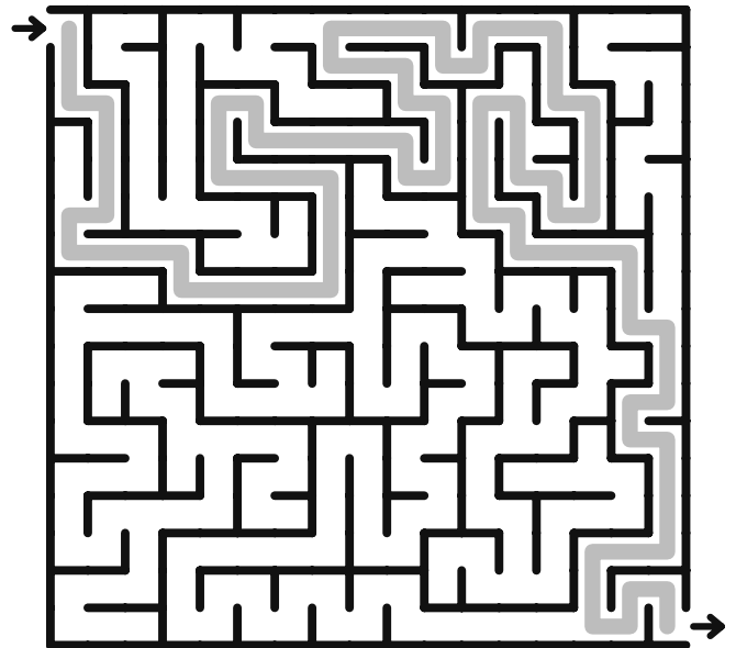
Maze 4
