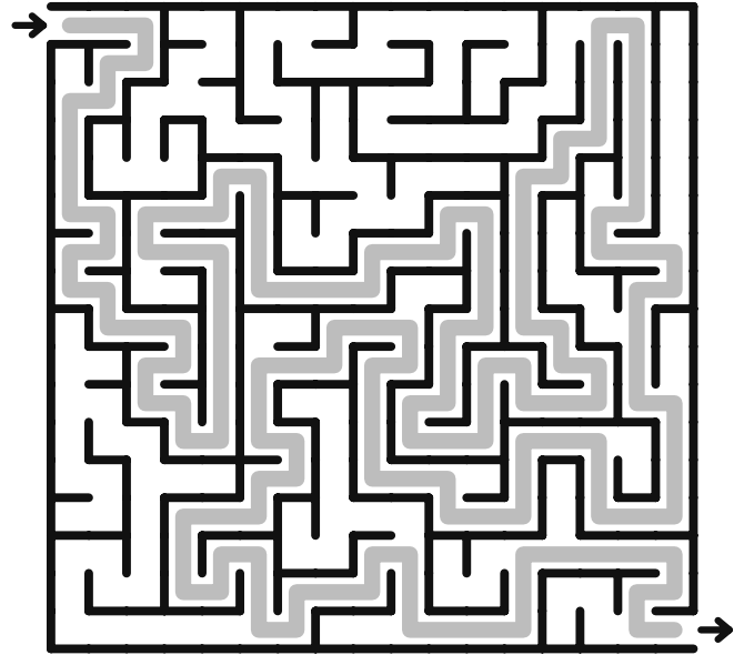
Maze 10
