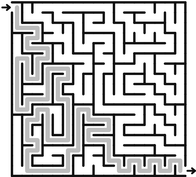
Maze 5
