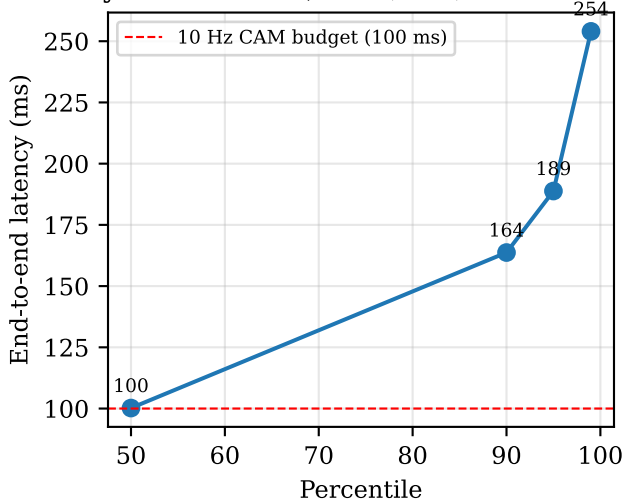
Latency Percentiles (n=10,000, mean=110.4 ms)
