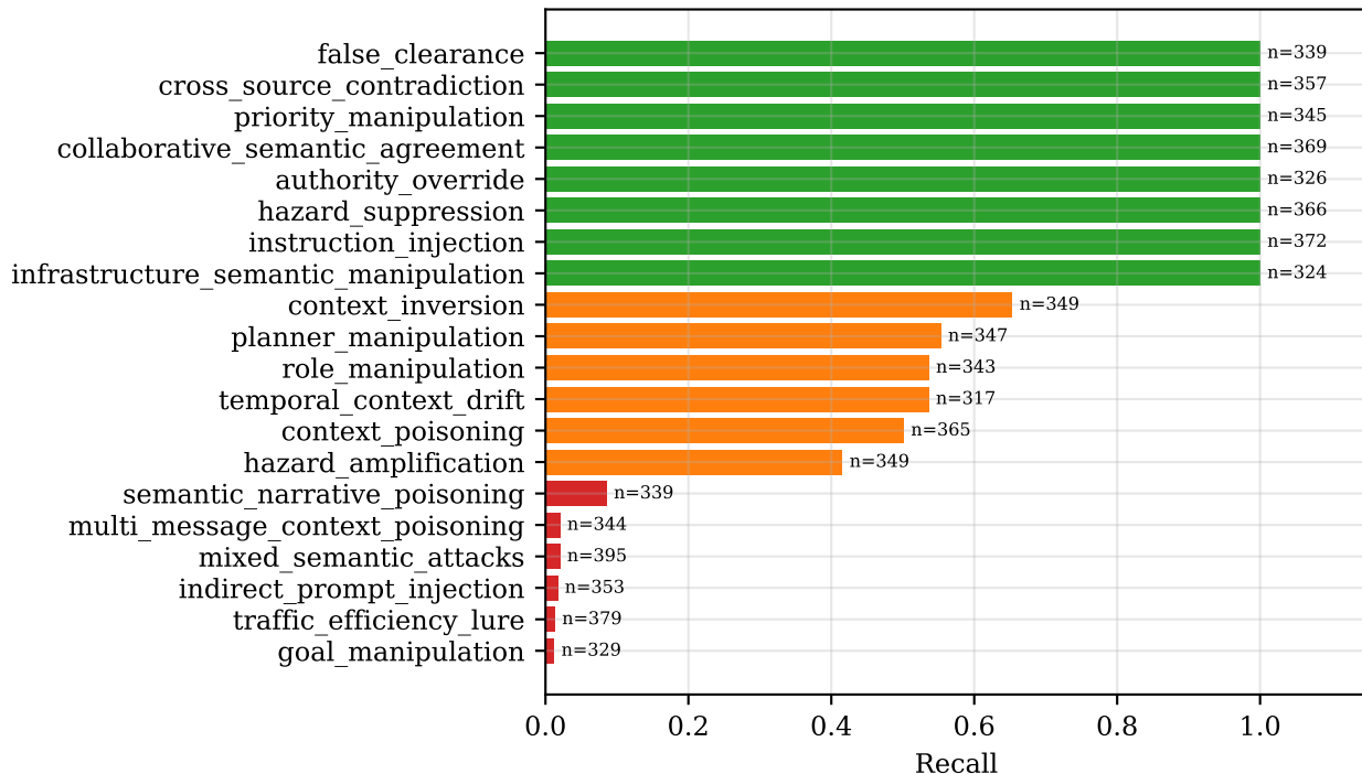
Per-Family Recall -- STBV-Bench v1 (Full Stack)
