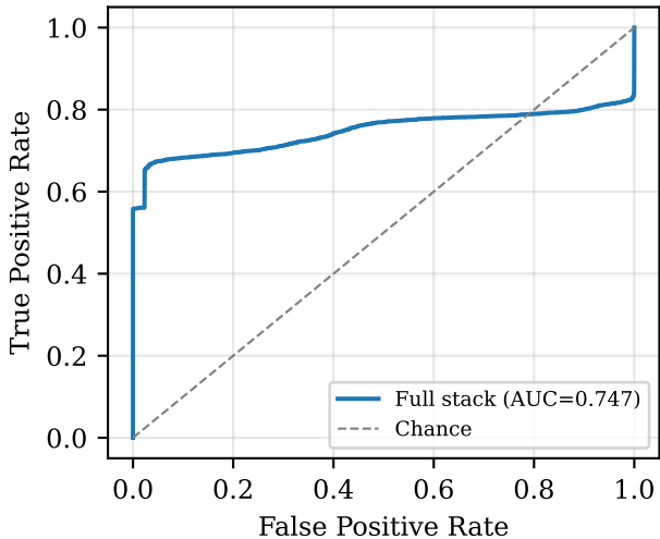
ROC -- STBV-Bench v1 ( n = 10,000 )
