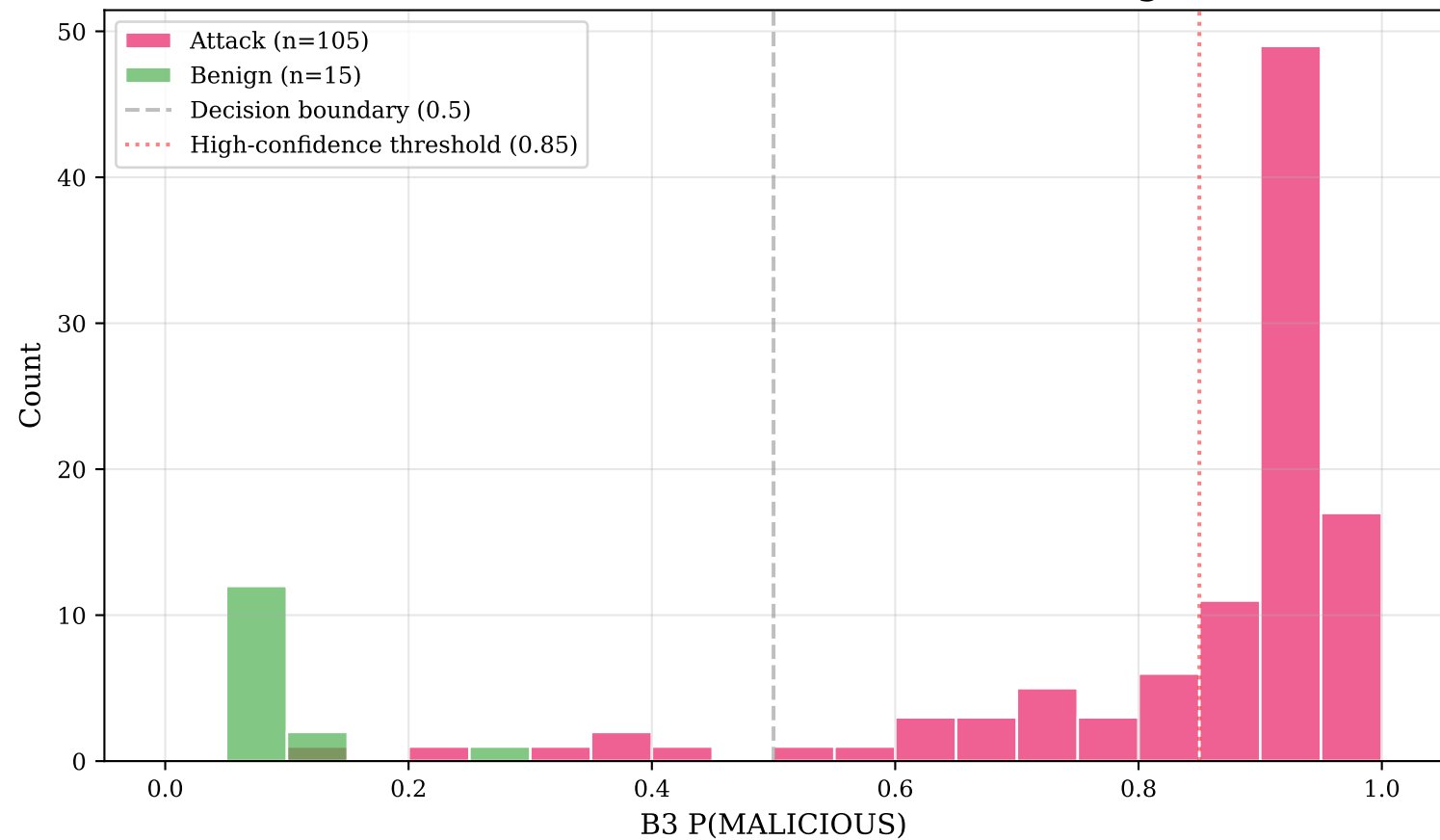
B3 Confidence Distribution — Attack vs Benign
