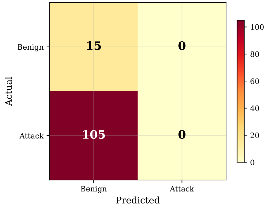
B1+B2 (Acc: 12.5%, F1: nan)
