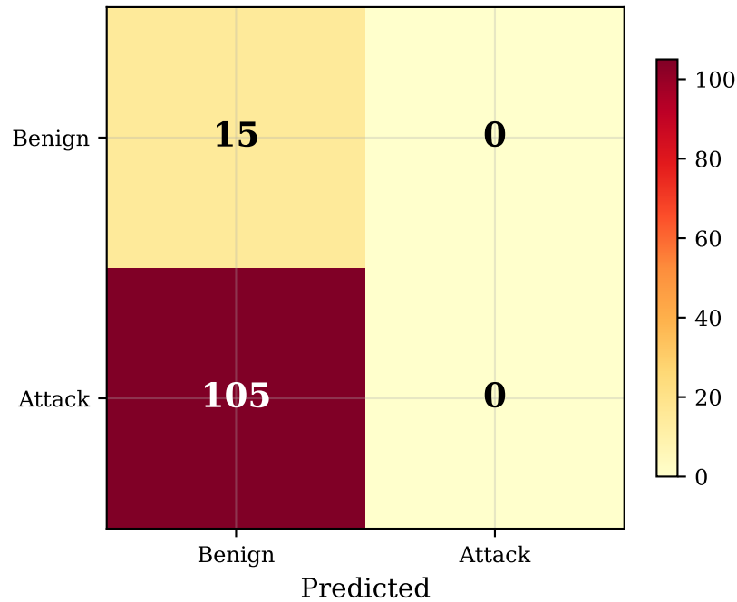
B1 Only (Acc: 12.5%, F1: nan)
