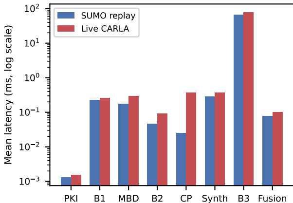
Per-stage latency: replay vs. live CARLA
