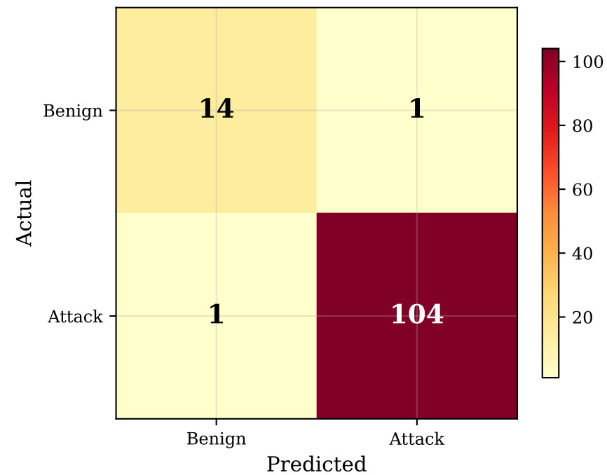
B1+B2+B3 (Acc: 98.3%, F1: 0.990)
