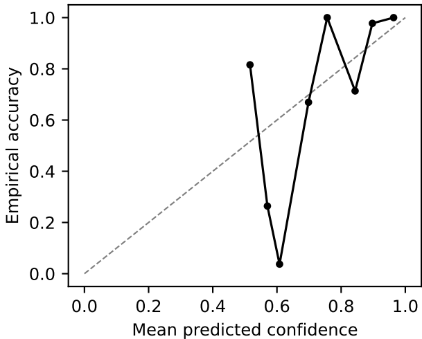
Calibration, STBV v1 (ECE=0.1533)
