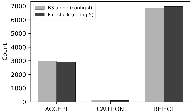
Decision Distribution Before/After Fusion, STBV v
