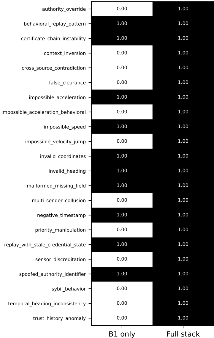
Per-Family Recall, ITE-Bench (Final Checkpoint)
