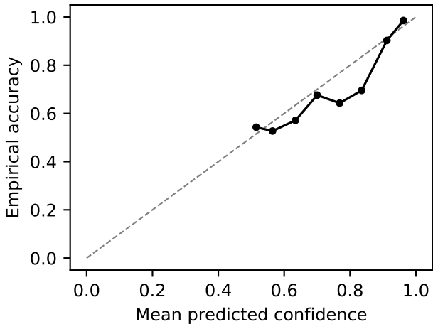
Calibration, STBV-Bench v2.5b ( T=3.18 , ECE=0.0268 )
