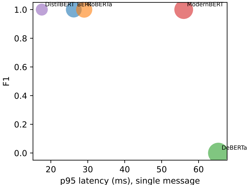
F1 vs. Latency (bubble size = peak VRAM)
