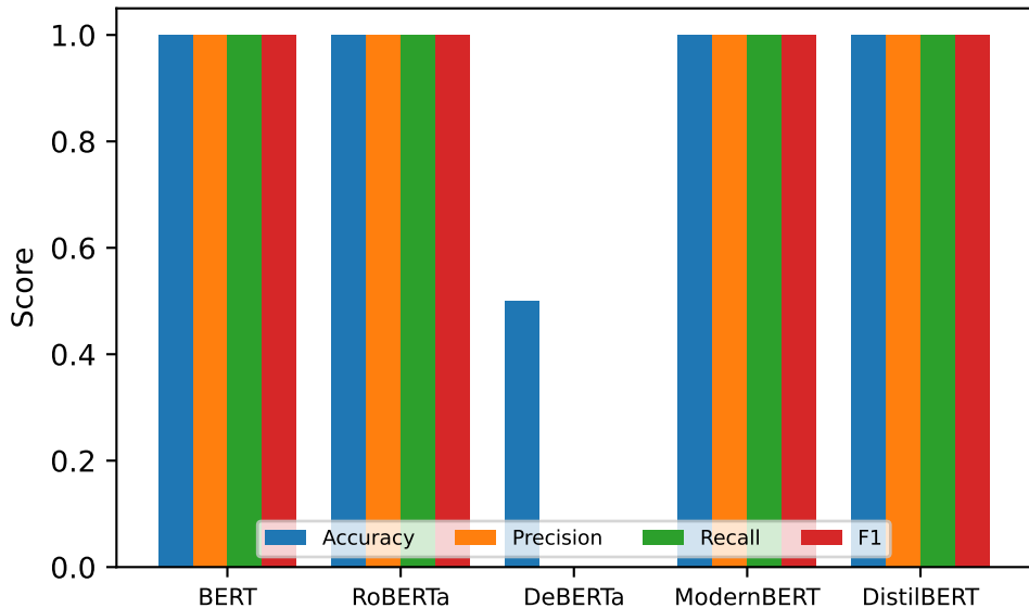
Classification Metrics by Backbone
